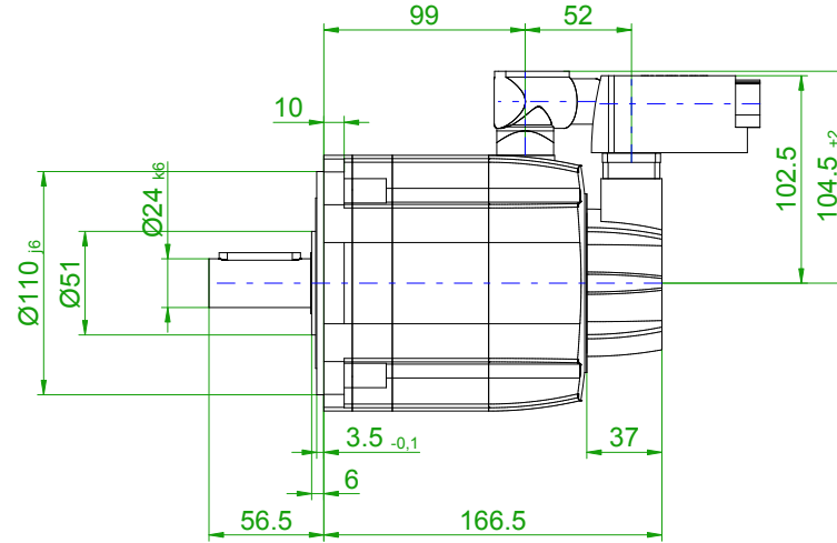
6-pole plug size 1 for power
