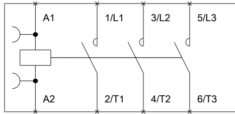
LEN00D & E Wiring Diagram
