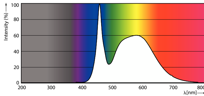
Spectral Power Distribution Colour - 19GC/LED/850/ND E26 BB 6/1
