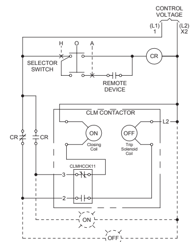
Connection for Hand/Off/Auto Control CLMOG and CLMOH
