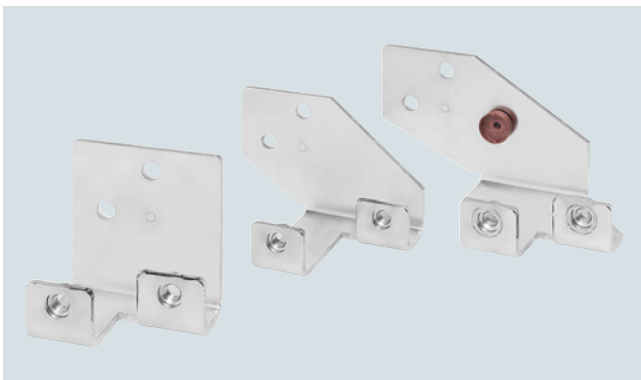
Installation kit for line-side cable connection, left, for SINAMICS G120X, frame size FSH
