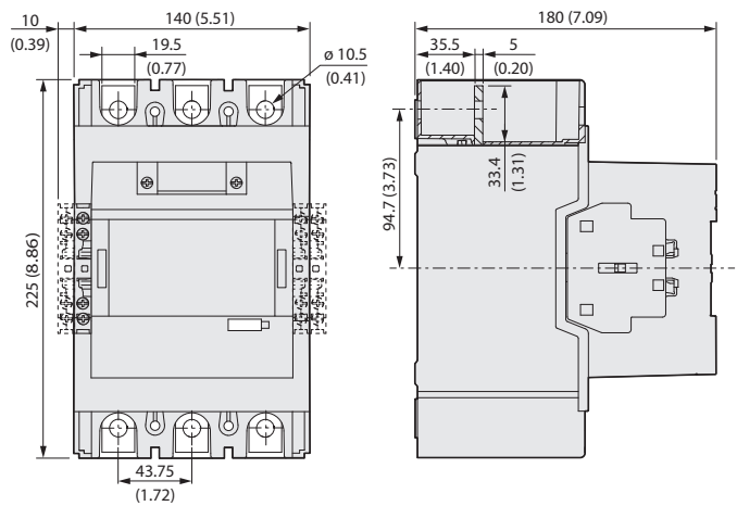
Figure 84 - 100-E265...100-E370 Contactors
