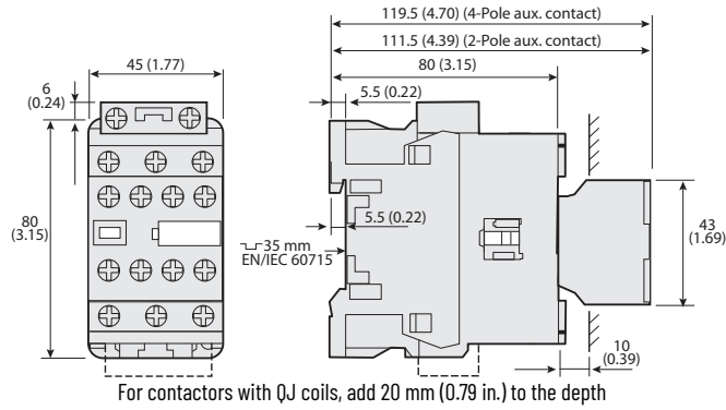
Figure 52 - 100-E26...100-E38 4-Pole Contactors with Low-consumption Coils and Front-mounted Auxiliary Contact
