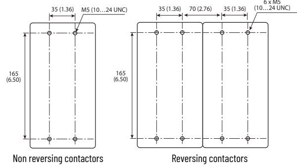
Figure 84 - 100-E265...100-E370 Contactors
