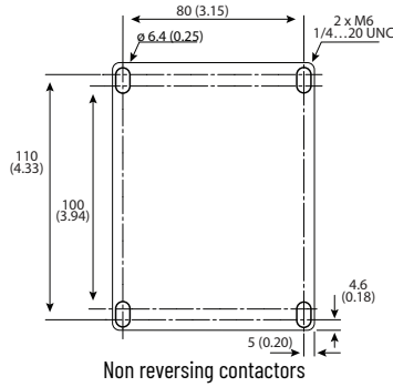
Figure 74 - Drilling Template for 80 A 4-Pole Contactors
