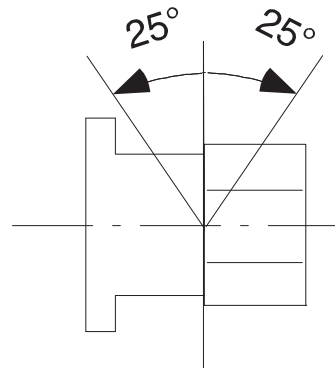
Figure 25 - Mounting Position – 100S-C DC Contactors with Conventional Coils
