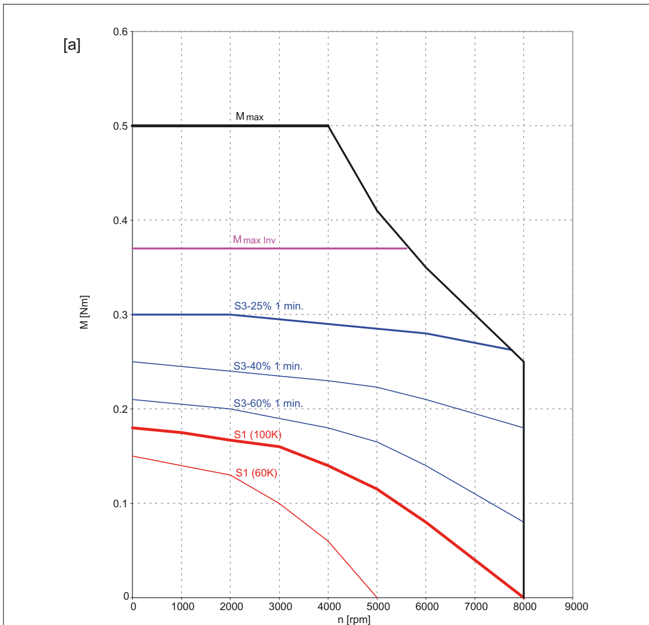
Figure 7-33 1FK7011-5AK21
