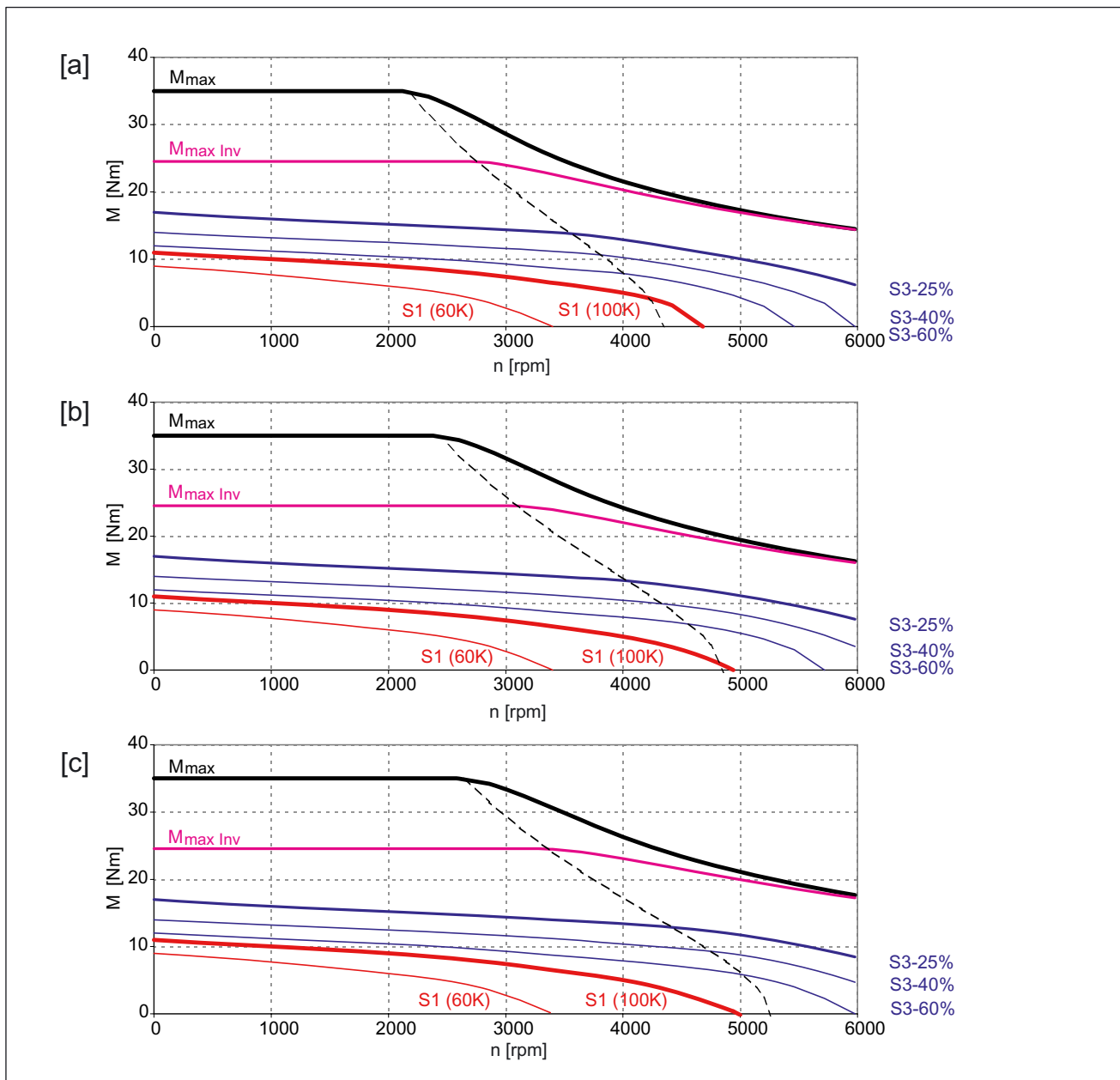
Figure 7-11 1FK7063-5AF71
