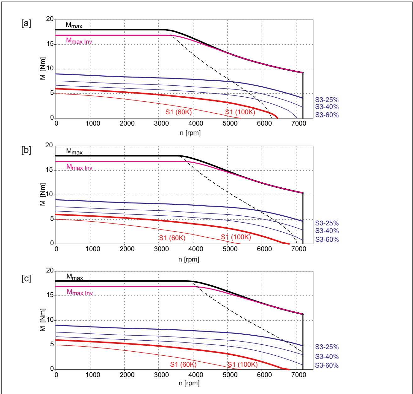
Figure 7-10 1FK7060-5AH71
