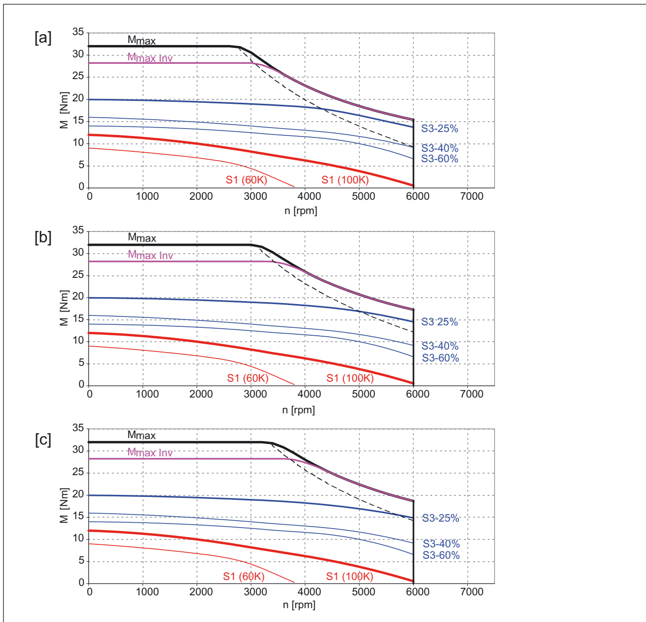
Figure 7-30 1FK7064-7AH71
