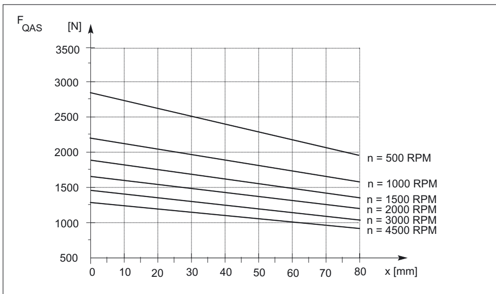
Figure 7-48 Cantilever force F_Q at a distance x from the shaft shoulder for a nominal bearing lifetime of 20,000 h.
