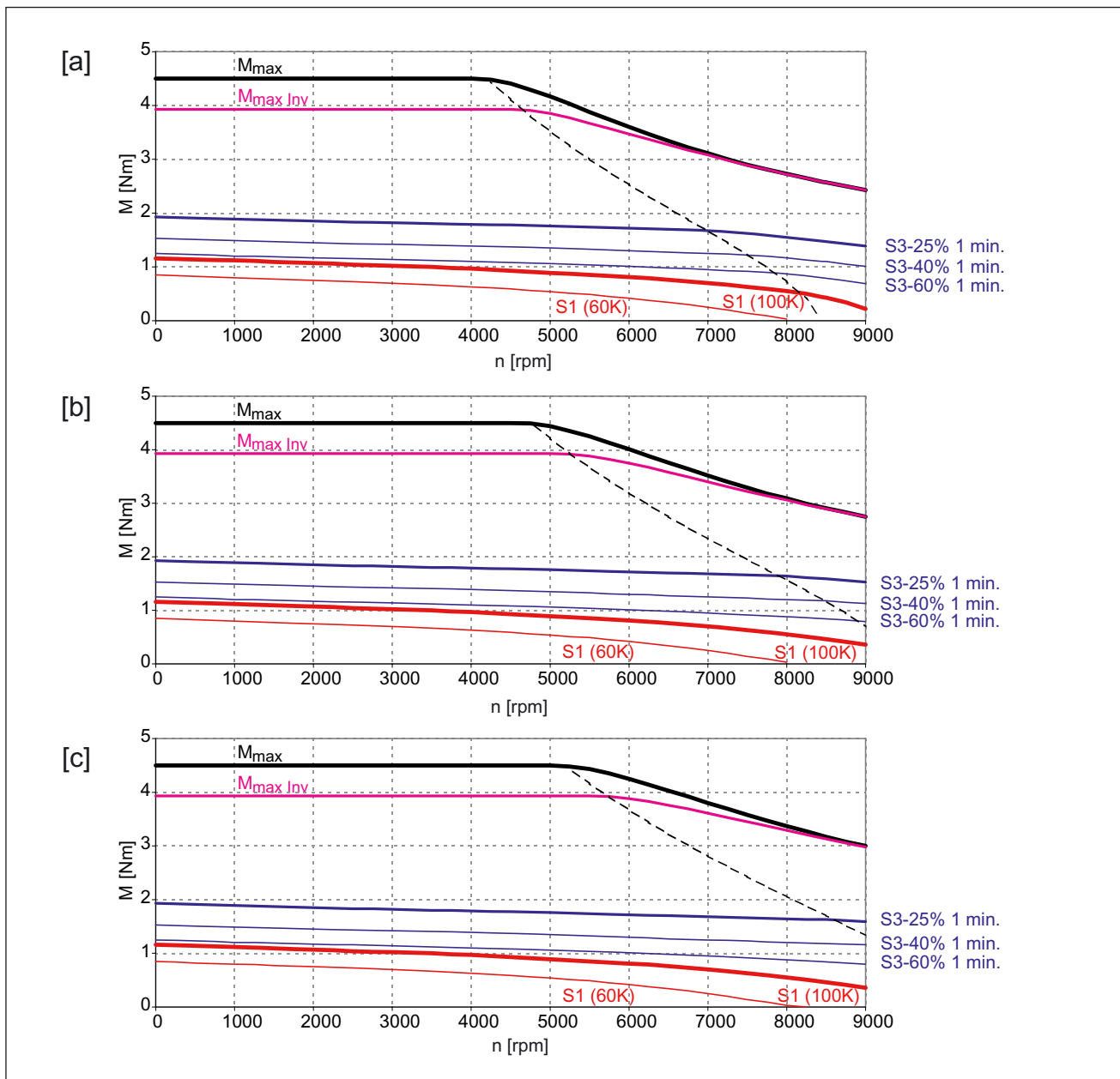
Figure 7-4 1FK7032-5AK71
