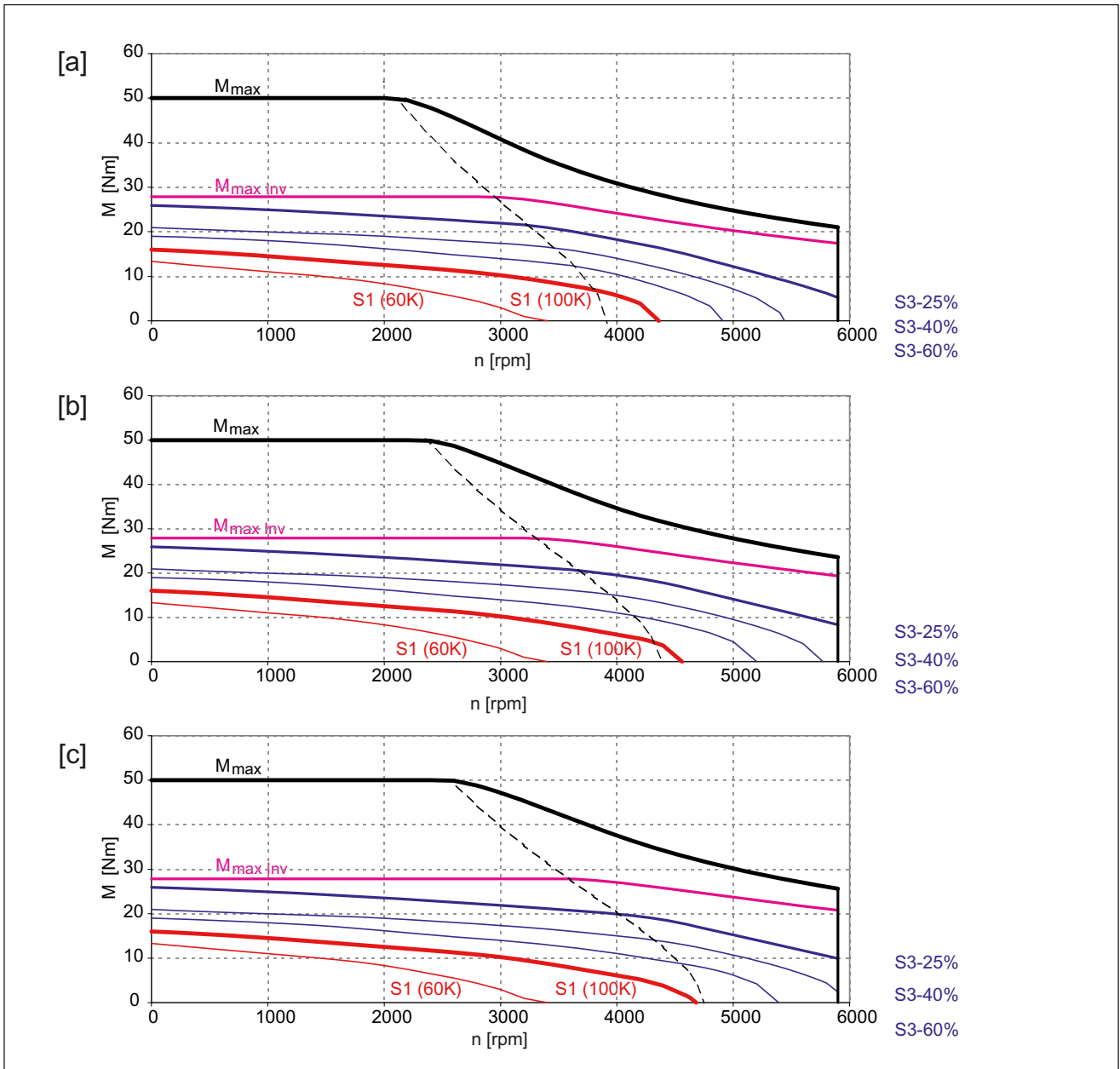
Figure 7-15 1FK7083-5AF71
