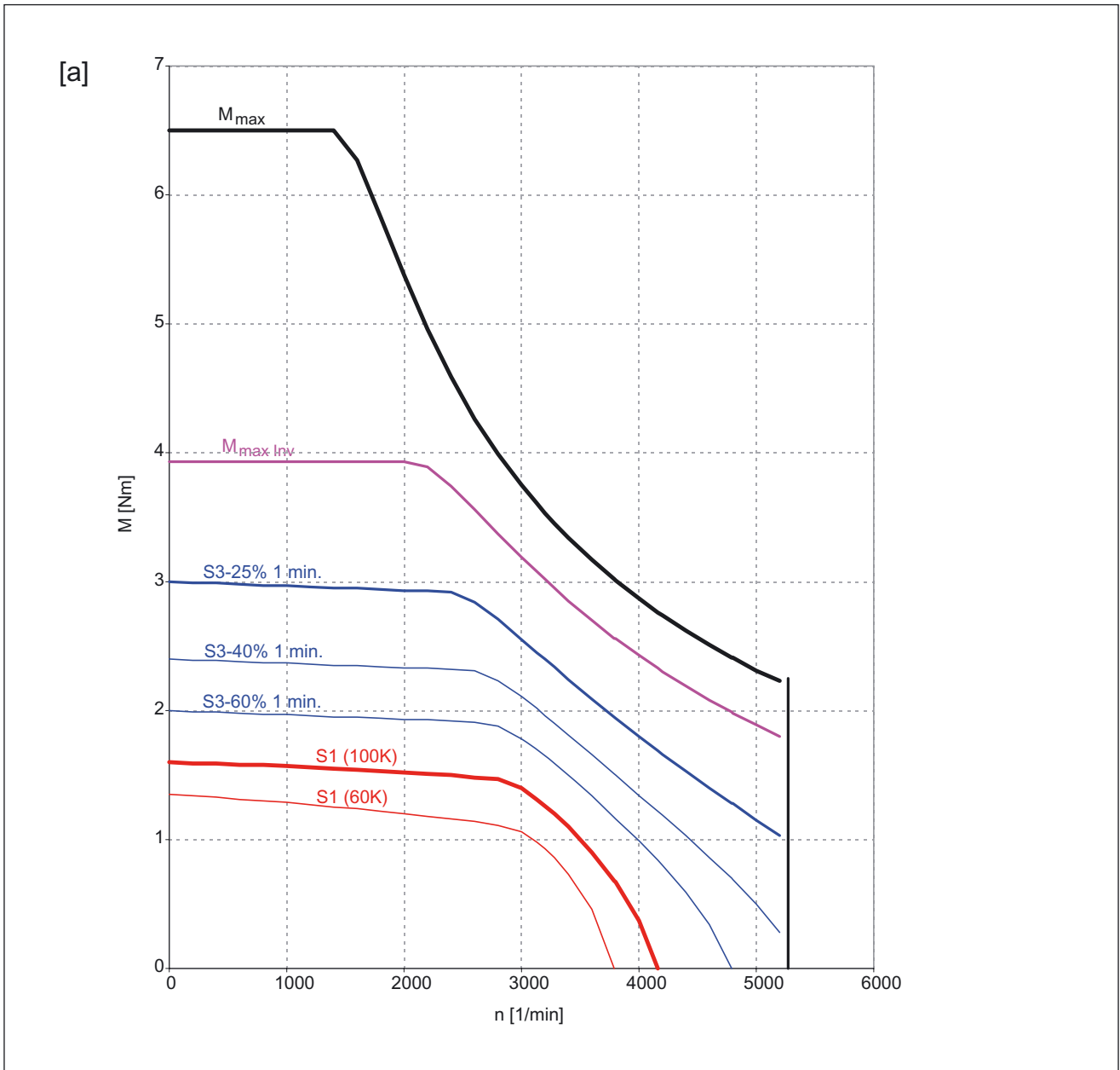
Figure 7-38 1FK7034-5AF21
