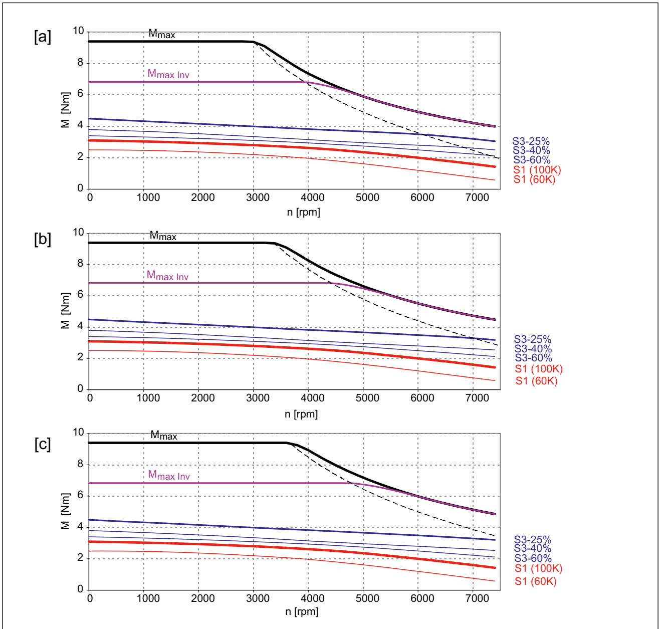
Figure 7-23 1FK7043-7AH71
