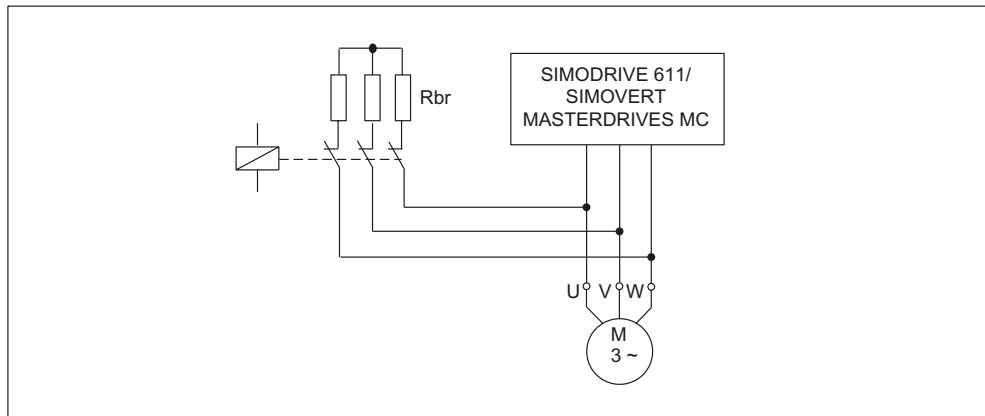
Figure 6-6 Circuit (schematic) with brake resistors
