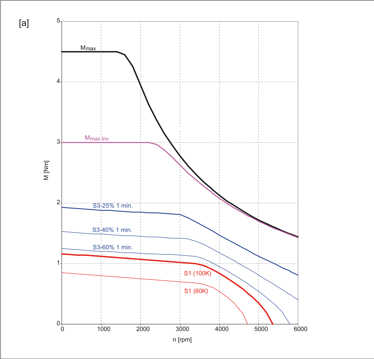
Figure 7-36 1FK7032-5AF21
