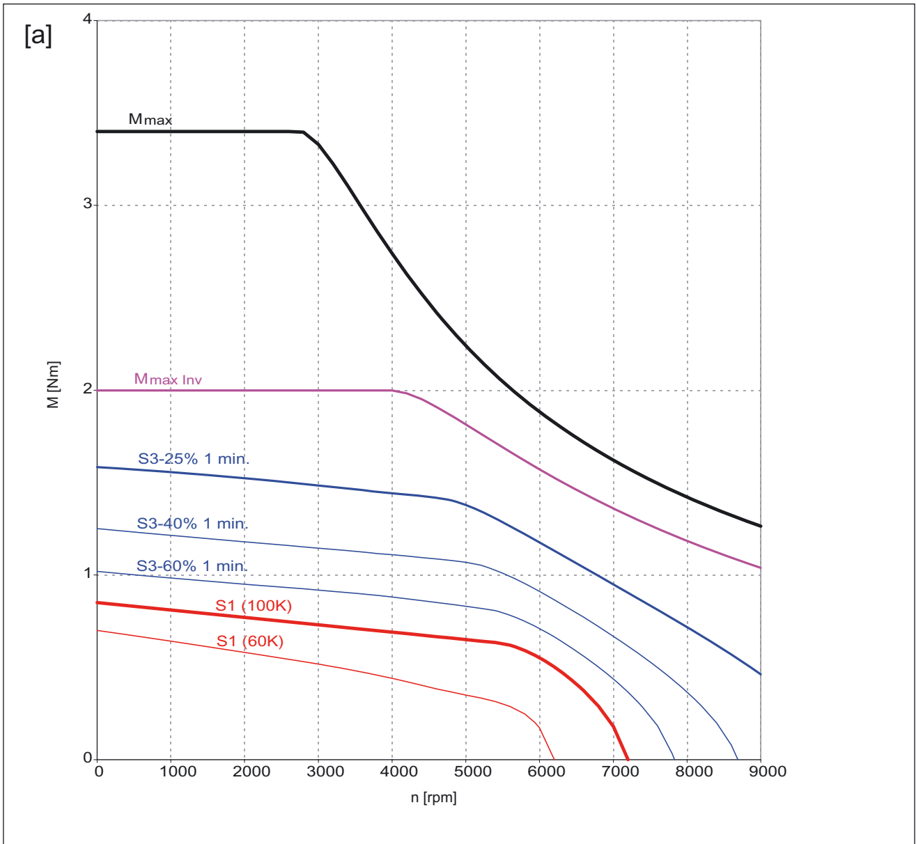
Figure 7-35 1FK7022-5AK21
