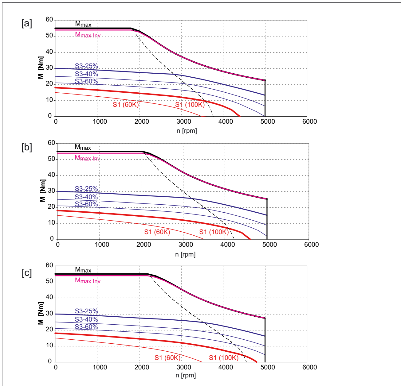
Figure 7-17 1FK7100-5AF71
