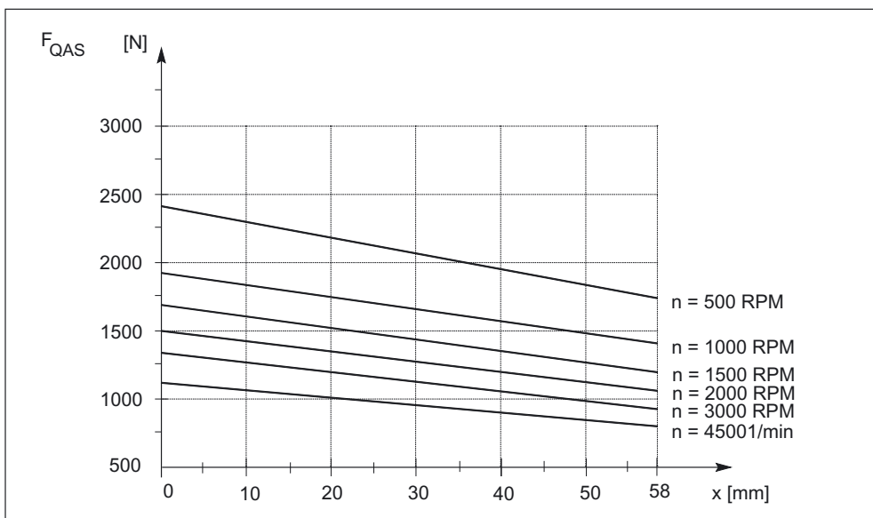
Figure 7-47 Cantilever force F_Q at a distance x from the shaft shoulder for a nominal bearing lifetime of 20,000 h.
