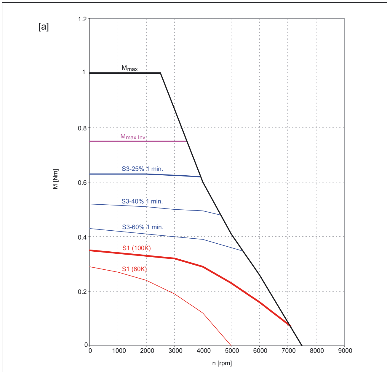
Figure 7-34 1FK7015-5AK21
