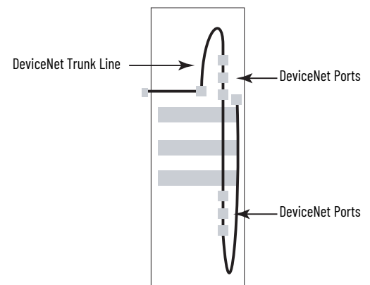
Inside look at DeviceNet cable routing in one CENTERLINE 2100 MCC section.
