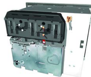
Shutters closed is 'disengaged' so the unit can be removed
