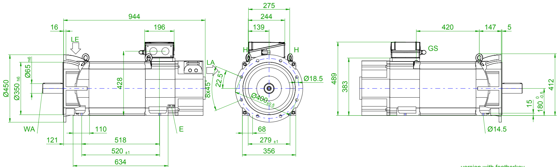
version with featherkey
