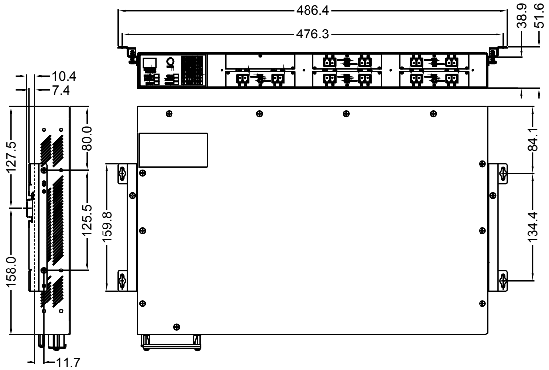
Figure 25: Panel and DIN Rail Mount Dimensions
