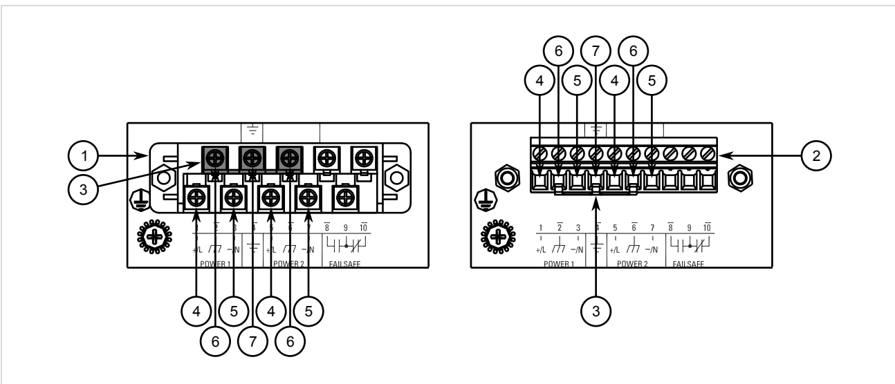
Figure 6: Terminal Block Wiring
