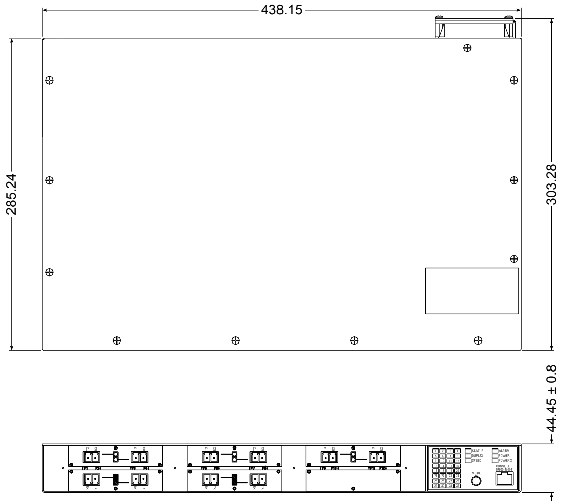
Figure 23: Overall Dimensions
