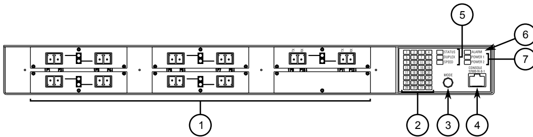
Figure 1: RUGGEDCOM RSG2200
