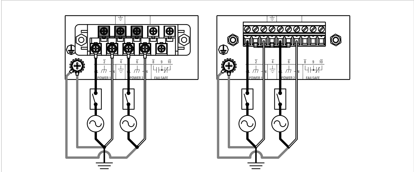
Figure 10: Dual AC Power Supply
