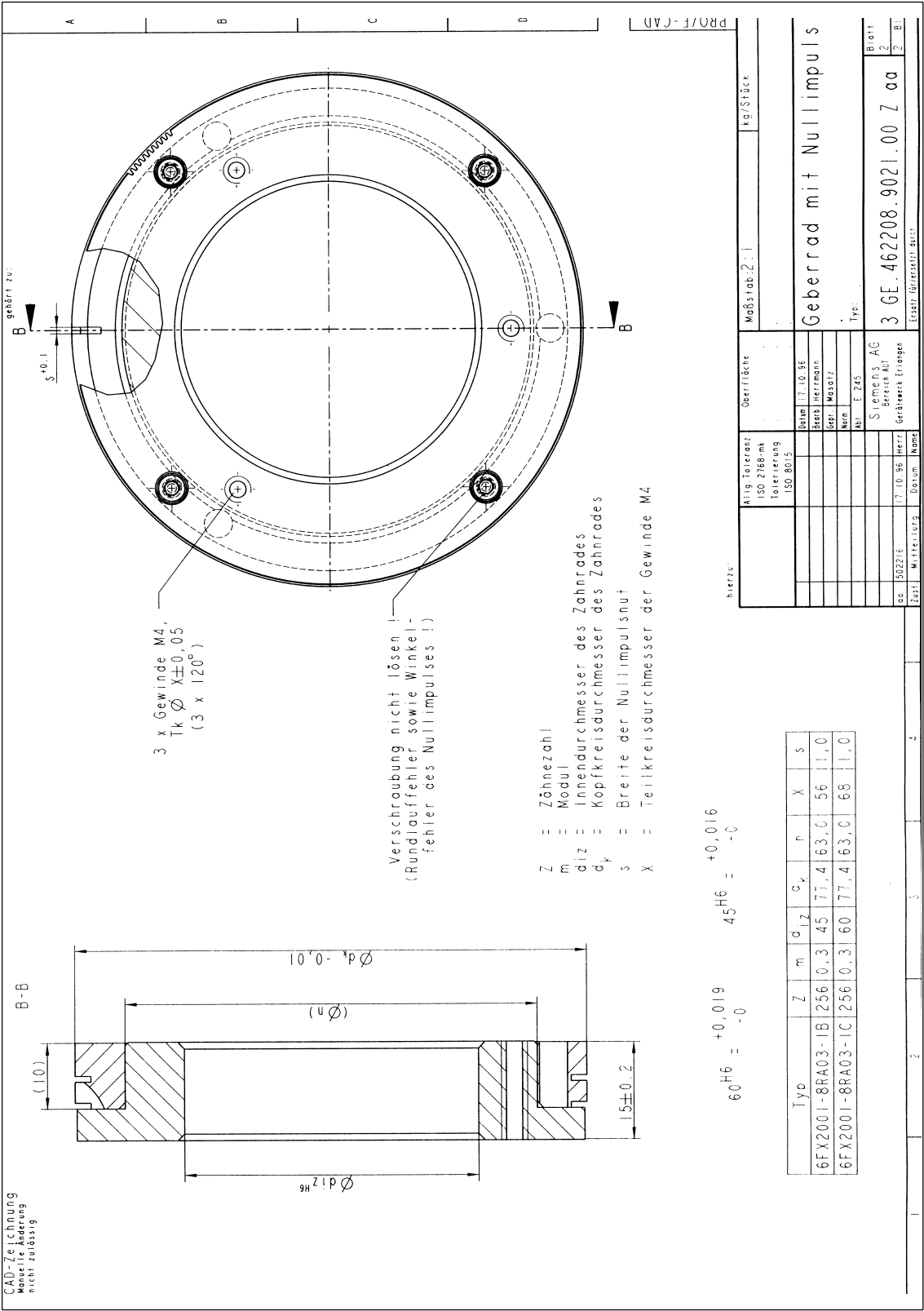
Fig. 4-5 Encoder wheel with zero pulse
