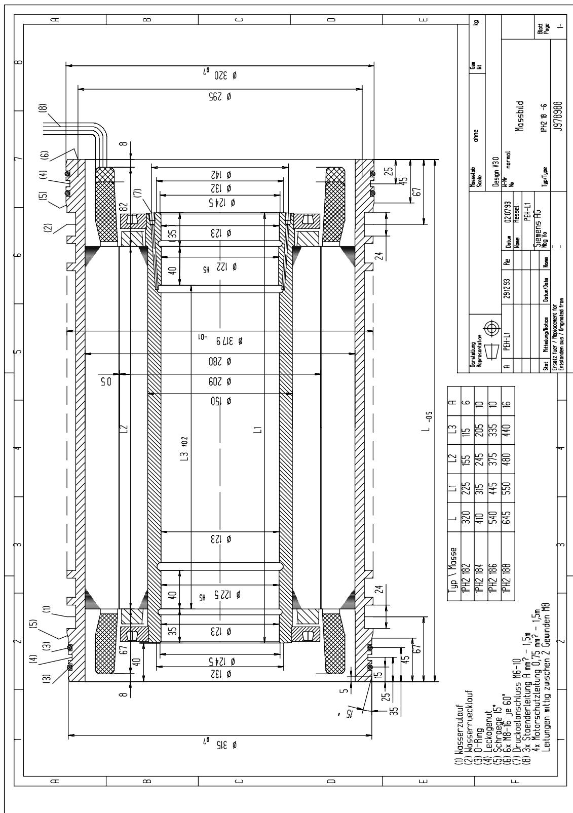
Fig. 5-7 1PH218□-6W motor dimensions (dimension drawing)
