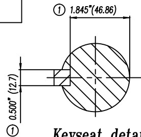
Keyseat detail Detalle Cuñero
