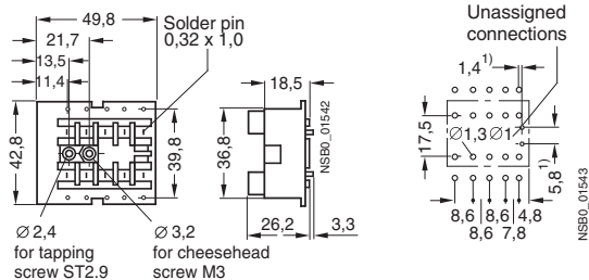
Hole pattern for plug-in base
