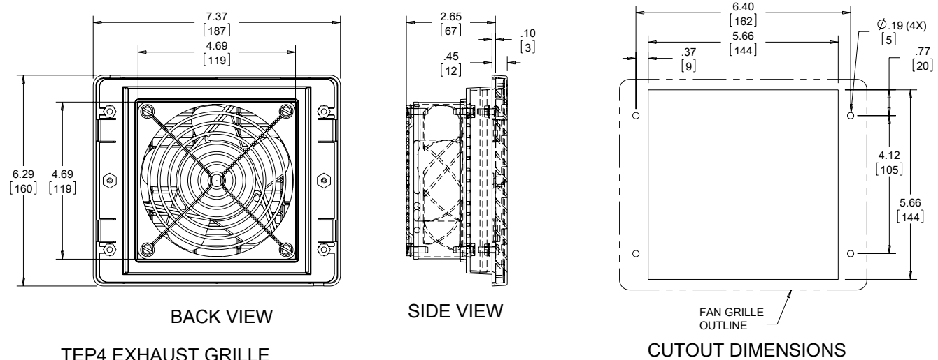
TEP4 EXHAUST GRILLE
