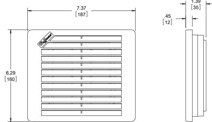
TEP4 EXHAUST GRILLE
