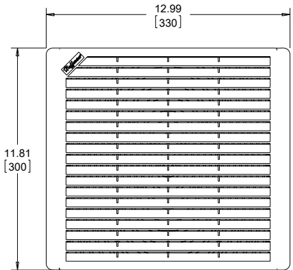
TEP10 EXHAUST GRILLE
