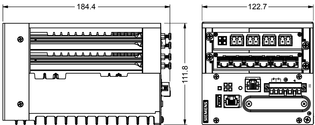
Figure 5.1 Overall Dimensions
