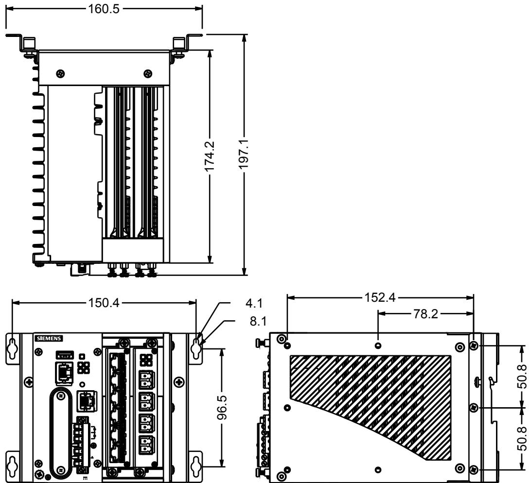
Figure 5.2 Panel and Din Rail Mount Dimensions
