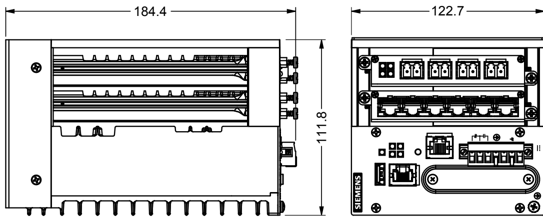
Figure 13: Overall Dimensions
