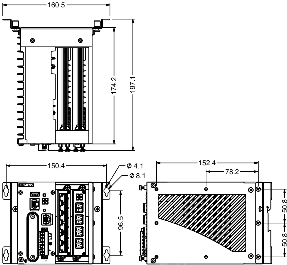
Figure 14: Panel and Din Rail Mount Dimensions
