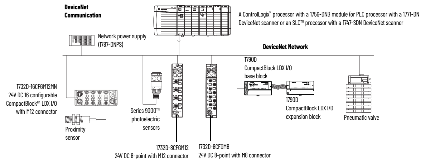
Figure 1 - DeviceNet Linear Topology Example
