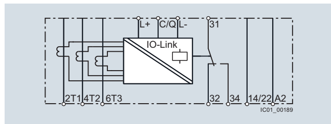
3RR2441-1AA40
