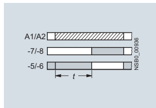
3RT1926-2E ON-delay
