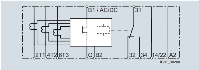
3RR2241-1F.30
