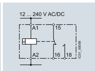
7PV1508-1AW30 Passing make contact
