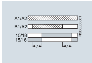
C 1) 3RP2005-.A ON-delay and OFF-delay with control signal ( t = t_{on} = t_{off} )
