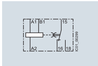
3RP2505-.A (C) ON-delay/OFF-delay with control signal
