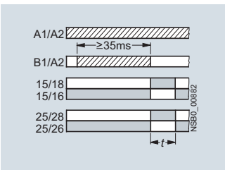
Retriggerable interval relay with deactivated control signal (passing break contact with control signal)
