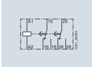
3RP2525-B ON-delay
