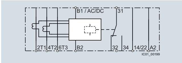
3RR2141-1A.30
