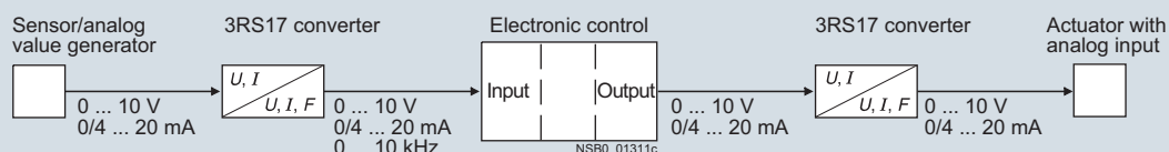
Application example: Interface converter in analog signal evaluation
