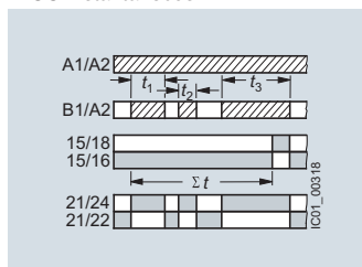
Additive ON-delay, instantaneous OFF with control signal and instantaneous contact
