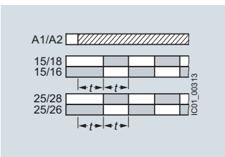
Flashing, symmetrical, starting with interval
