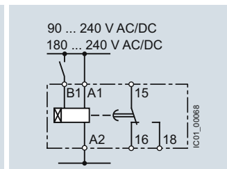
7PV1518-1AJ30, 7PV1518-1AN30 ON-delay
