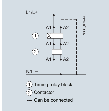
3RT1926-2C ON-delay
