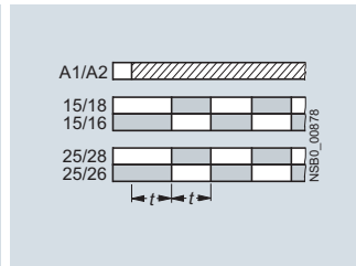
Flashing, symmetrical, starting with pulse
