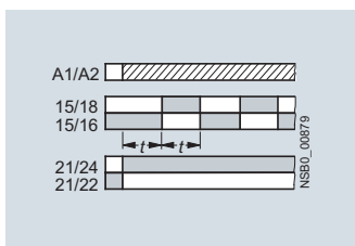
D• 3RP2005-.B Flashing, starting with interval (pulse/interval 1:1) and instantaneous contact
