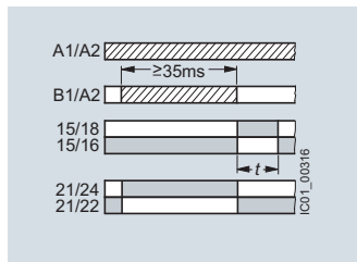
Retriggerable interval relay with deactivated control signal (passing break contact with control signal) and instantaneous contact
