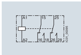
3RP2505-.B (K) Pulse-delayed (fixed pulse (at 1 s) and settable pulse delay)
