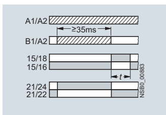
F•¹) 3RP2005-.B Passing break contact with control signal and instantaneous contact
