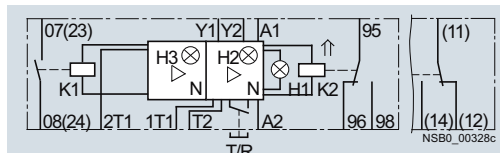
3RN1022
