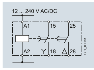
7PV1578-1BW30 Wye-delta
