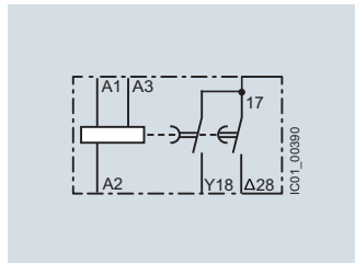
3RP257. Wye-delta function
