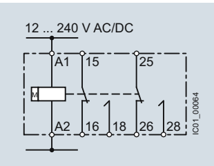
7PV1508-1BW30 Passing make contact
