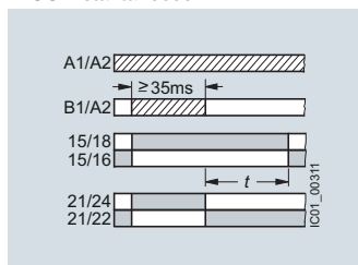
OFF-delay with control signal and instantaneous contact
