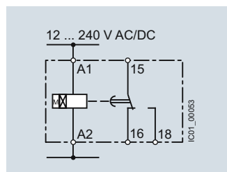
7PV1508-1AW30 ON-delay
