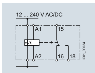
7PV1508-1AW30 Flashing, starting with interval
