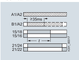
Passing make contact with control signal, not retriggerable (pulse-forming with control signal) and instantaneous contact
