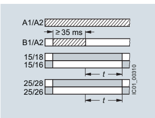
OFF-delay with control signal
