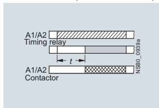
3RT1926-2C ON-delay two-wire design (varistor integrated)
