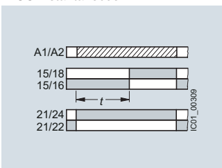
ON-delay and instantaneous contact
