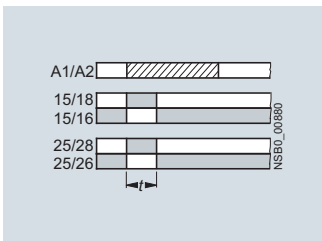
Passing make contact, interval relay
