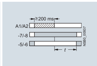
3RT1926-2F OFF-delay without control signal
