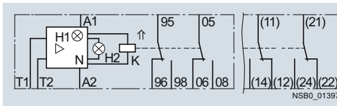
3RN1010, 2 CO
