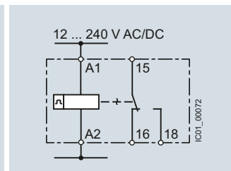
7PV1558-1AW30 Clock-pulse relay
