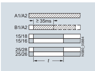
Passing make contact with control signal, not retriggerable (pulse-forming with control signal)
