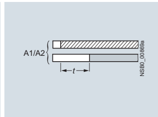
3RP2527..-EW30, 1 NO (semiconductor), ON-delay
