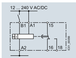
7PV1508-1AW30 Additive ON-delay, with control signal
