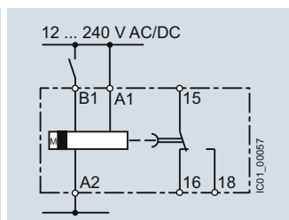
7PV1508-1AW30 OFF-delay
