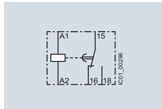
3RP2505-.A (A) ON-delay
