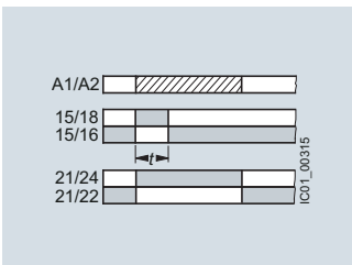
Passing make contact, interval relay and instantaneous contact
