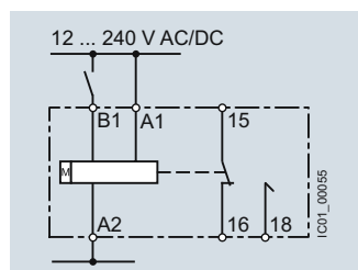
7PV1508-1AW30 Passing break contact with control signal
