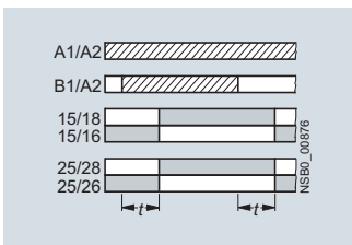
ON-delay/OFF-delay with control signal
