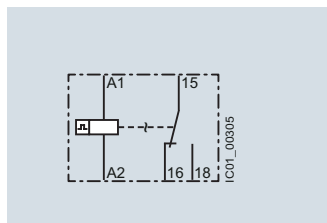
3RP2505-.A (J) Flashing, symmetrical, starting with pulse
