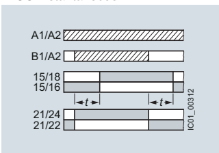
ON-delay/OFF-delay with control signal and instantaneous contact
