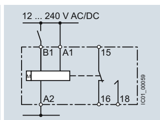
7PV1508-1AW30 Pulse-forming with control signal
