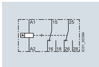
3RP2505-.B (J) Flashing, symmetrical, starting with pulse
