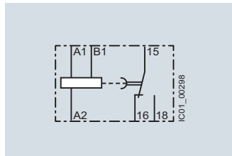
3RP2505-.A (B) OFF-delay with control signal
