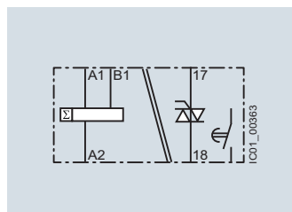
3RP2505-.C (H) Additive ON-delay, instantaneous OFF with control signal
