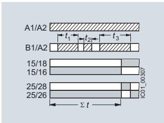
Additive ON-delay with control signal
