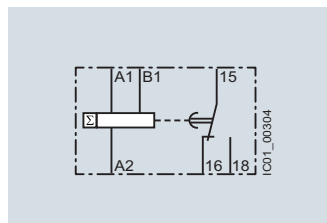
3RP2505-.A (I) Additive ON-delay with control signal
