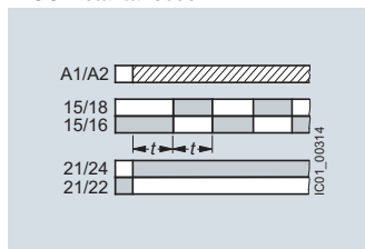
Flashing, symmetrical, starting with interval and instantaneous contact
