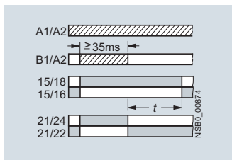
B•¹) 3RP2005-.B OFF-delay with control signal and instantaneous contact
