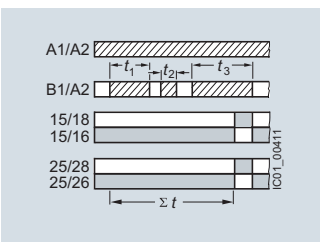
Additive ON-delay, instantaneous OFF with control signal
