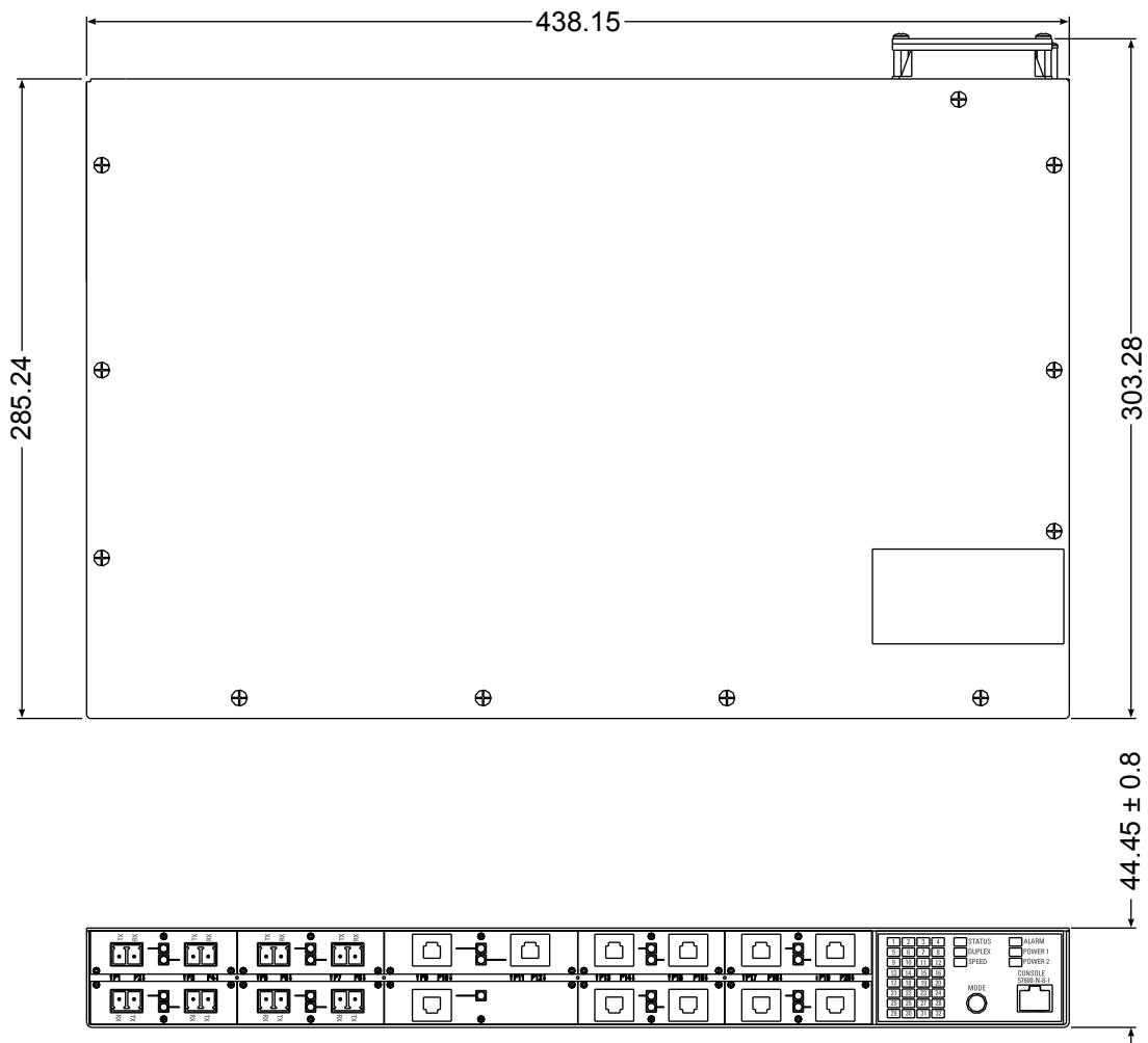
Figure 29: Overall Dimensions
