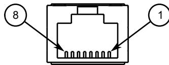
Figure 19: RJ45 Ethernet Port Pin Configuration
