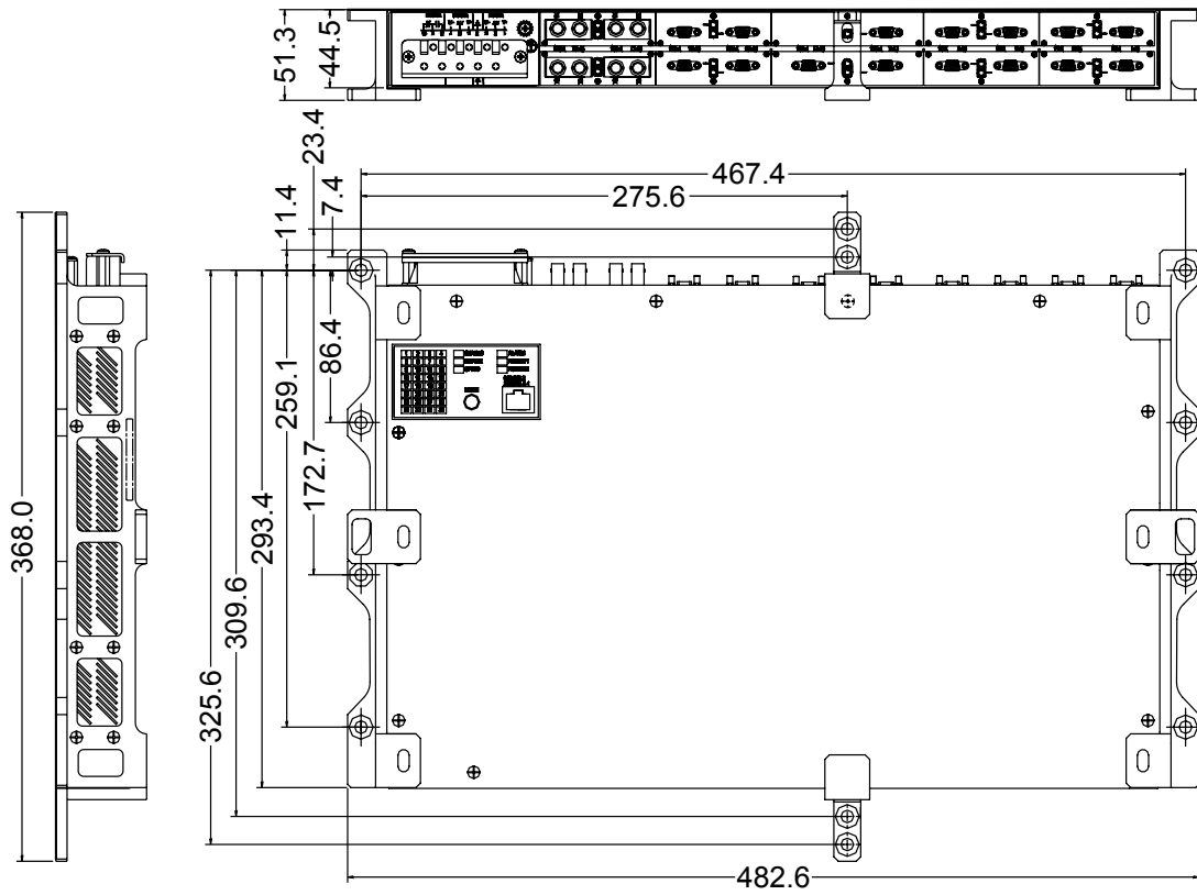
Figure 31: Panel Mount Dimensions
