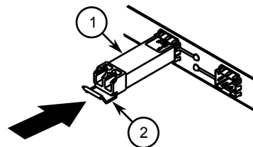
Figure 26: Installing an SFP Optical Port (Typical)
