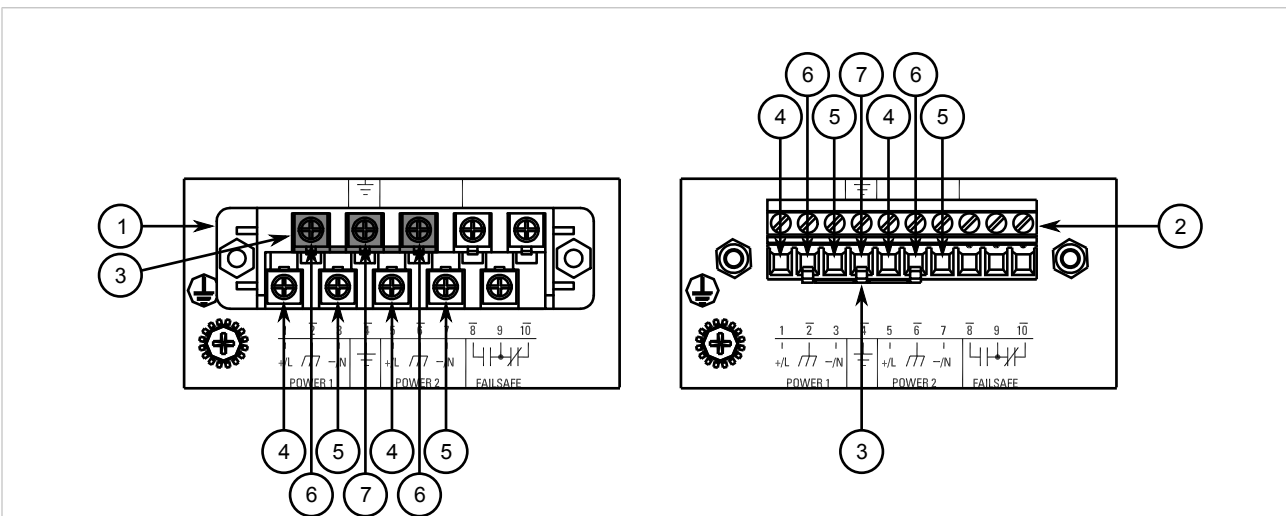
Figure 5: Terminal Block Wiring
