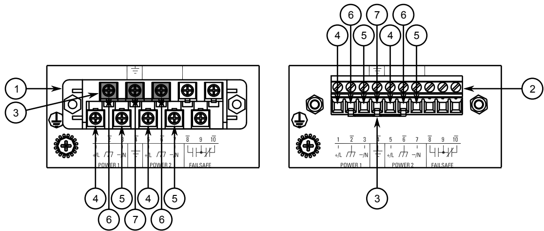
Figure 4: Terminal Block Wiring
