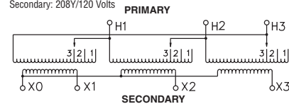
T600A Wiring Diagram & Connections*
