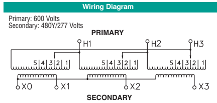
T600I Wiring Diagram & Connections*
