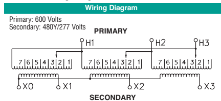
T600M Wiring Diagram & Connections*
