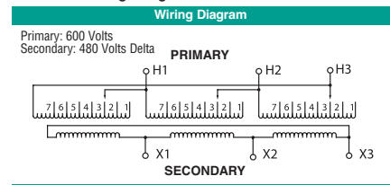
T600K Wiring Diagram & Connections*
