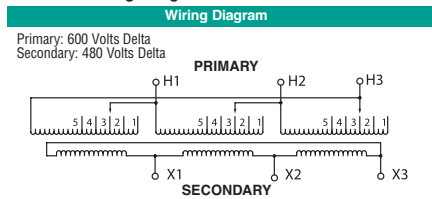
T600L Wiring Diagram & Connections*
