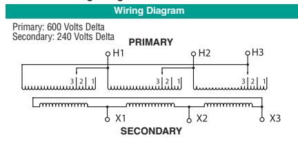
T600J Wiring Diagram & Connections*
