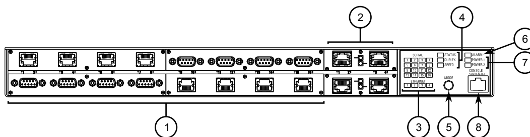
Figure 1: RUGGEDCOM RS416
