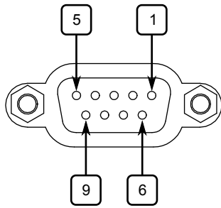
Figure 26: Serial DB9 Port Pin Configuration
