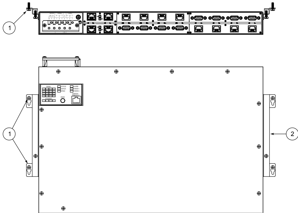
Figure 6: Panel Mounting
