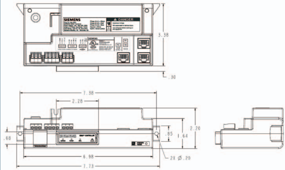
Controller Dimensions
