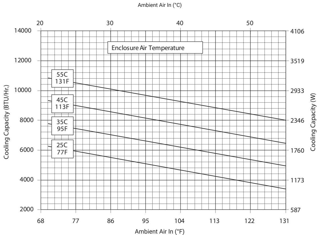
G52-0846-GXXX Capacity Curves at 50 Hz
