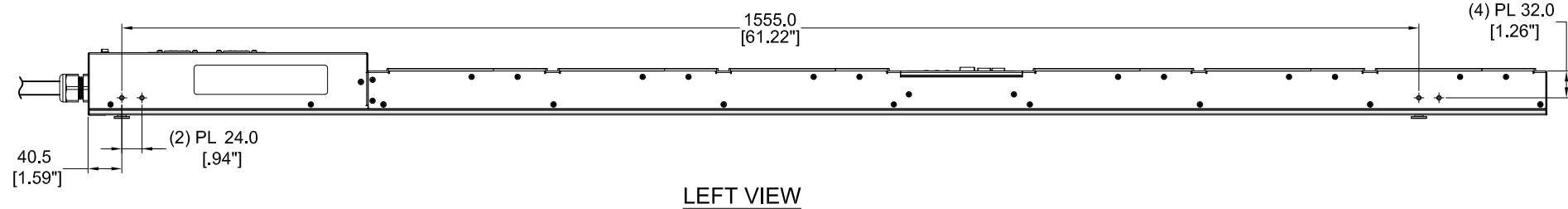
LEFT VIEW
