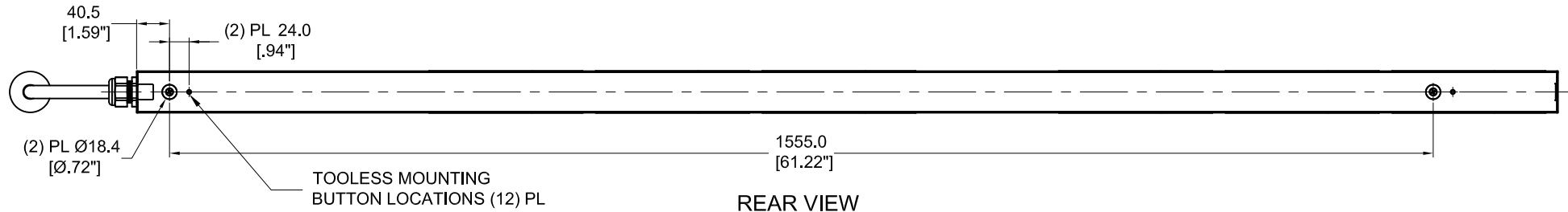
REAR VIEW
