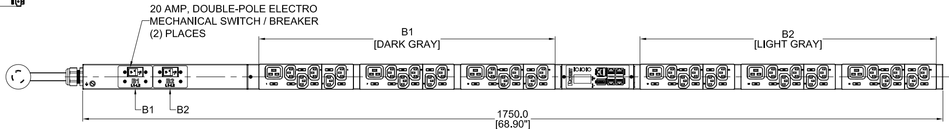
FRONT VIEW
