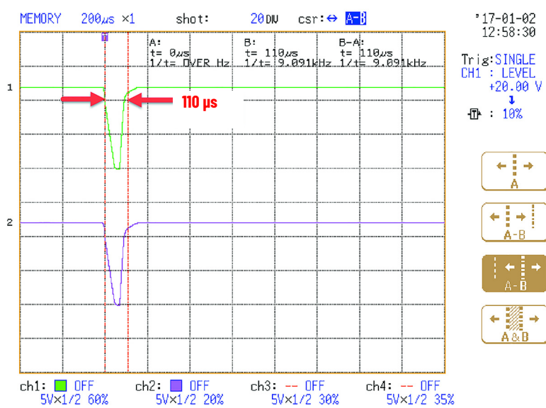
Figure 85 - OSSD Channel Transistor Test Pulse
