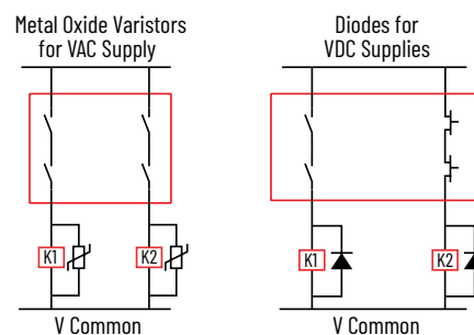
Figure 18 - Surge Suppressors
