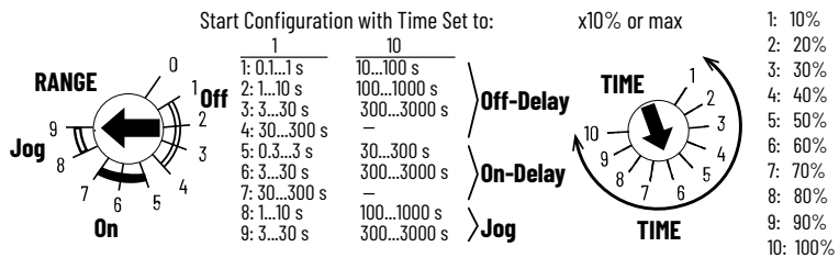
Figure 27 - EMD Safety Relay Range and Time
