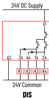
Figure 17 - OSSD Output Connections
