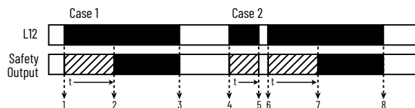
Figure 35 - On-delay Timing Diagram
