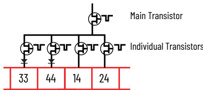
Figure 31 - Output Transistor Arrangement
