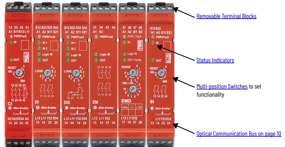
Figure 1 - Safety Relays
