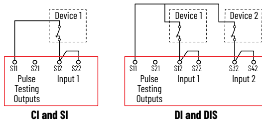
Figure 9 - Example Connections to 1 N.C. Mechanical Contact
