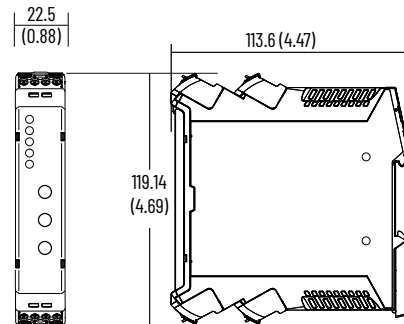
Figure 2 - Approximate Dimensions [mm (in.)]
