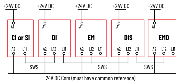
Figure 19 - Example SWS Connections
