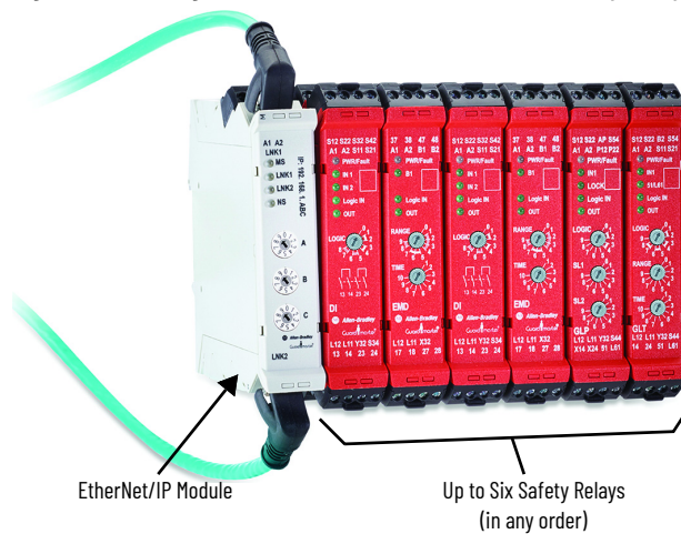
Figure 54 - Arrangement of EtherNet/IP Module and Safety Relays
