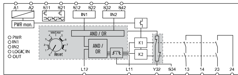
Figure 38 - DI Safety Relay Circuit Diagram
