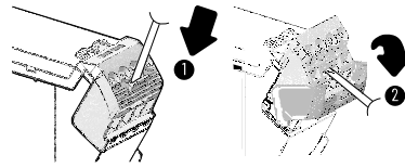
Figure 4 - Removable Terminals
