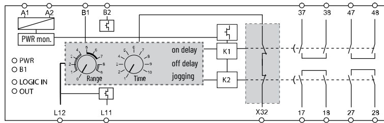
Figure 41 - EMD Safety Relay Circuit Diagram
