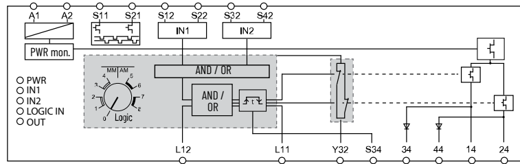
Figure 39 - DIS Safety Relay Circuit Diagram
