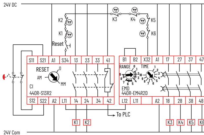
Figure 50 - EMD Safety Relay - Off Delay
