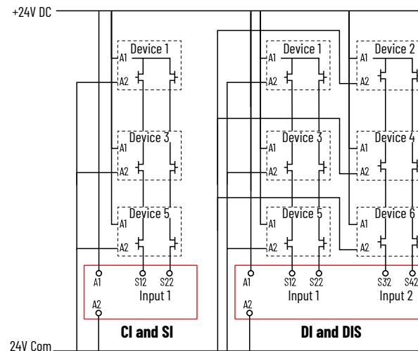
Figure 11 - Example Connections to Device with Cascaded and Non-cascaded OSSD Devices
