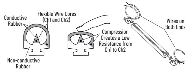
Figure 14 - Safedge Operating Principle
