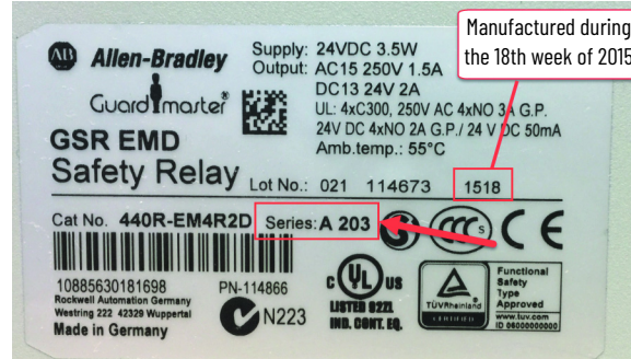
Figure 93 - Product Label - Series and Revision Identification
