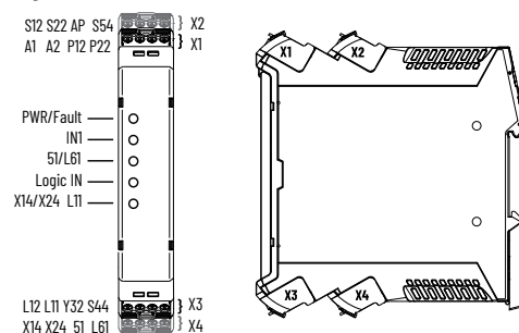
Figure 5 - Terminal Identification
