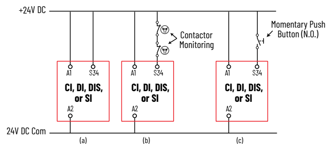
Figure 22 - Automatic/Manual Reset Connections
