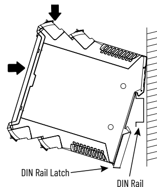
Figure 3 - DIN Rail Mounting
