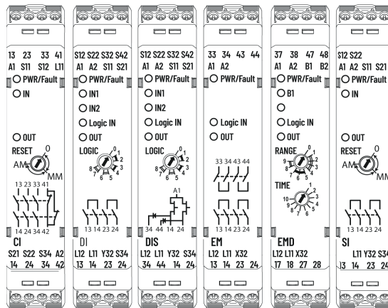
Figure 6 - Safety Relay Face Markings
