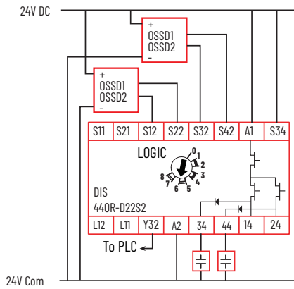
Figure 48 - High Capacitive Load
