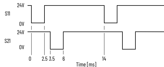
Figure 29 - Pulse Test Sequence for CI Safety Relay
