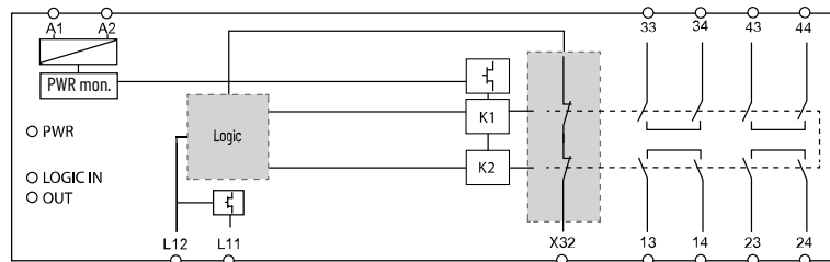
Figure 40 - EM Safety Relay Circuit Diagram
