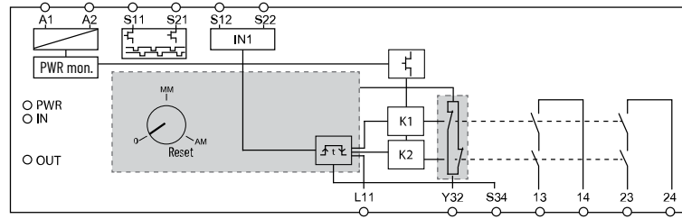
Figure 42 - SI Safety Relay Circuit Diagram
