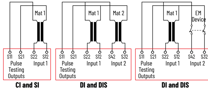
Figure 12 - Example One Connection to Safety Mats
