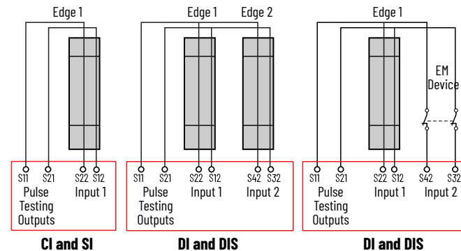
Figure 15 - Example Connections to Safety Edges
