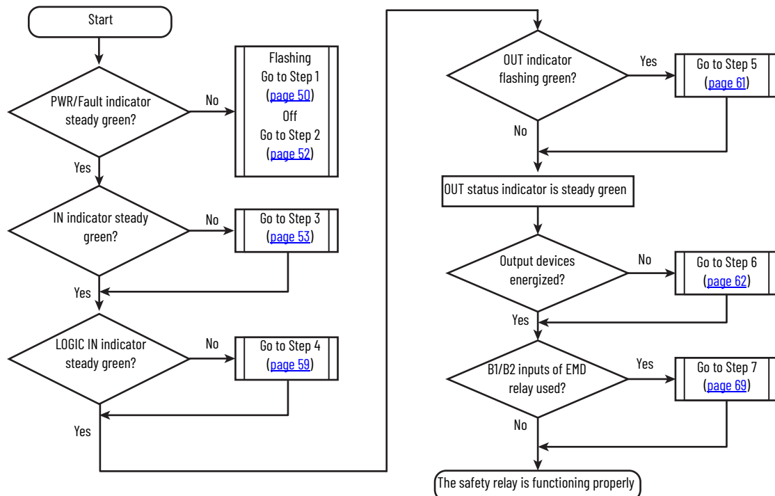
Figure 58 - Troubleshooting Flowchart
