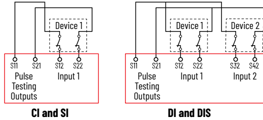
Figure 8 - Example Connections to 2 N.C. Mechanical Contacts
