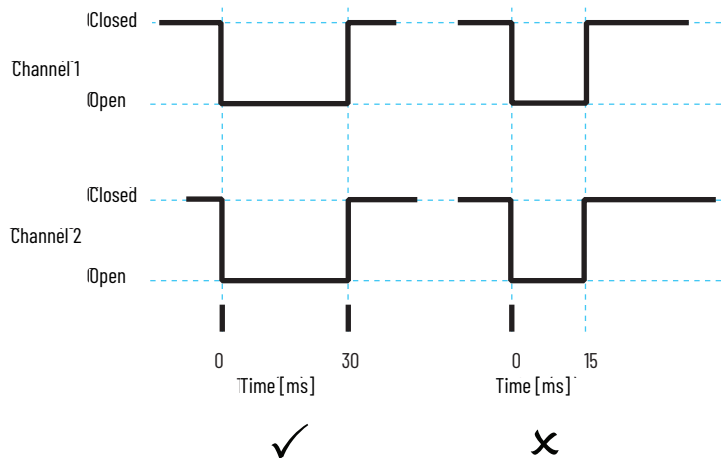
Figure 72 - Recovery Time
