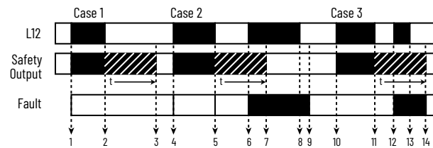
Figure 33 - Off-delay, Non-retriggerable Timing Diagram
