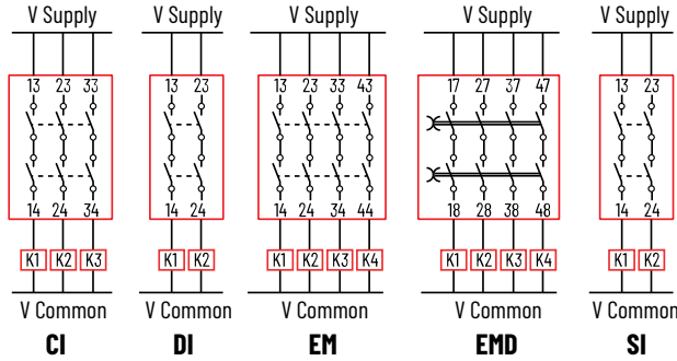
Figure 16 - Electromechanical Output Connections
