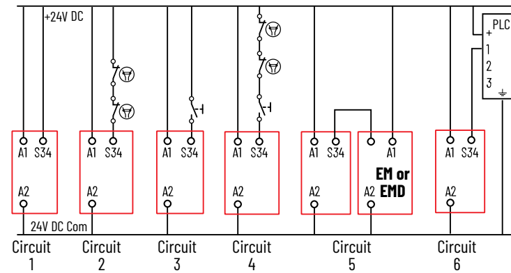
Figure 21 - Typical Reset/Monitoring Circuits
