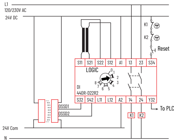
Figure 46 - With a Safety Mat and Device with OSSD Outputs, Monitored Manual Reset, AC Loads
