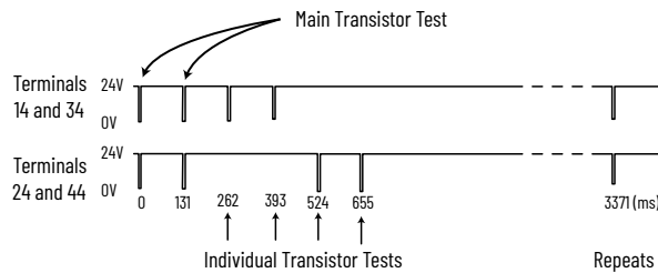
Figure 32 - OSSD Output Test Pulses on DIS Safety Relay
