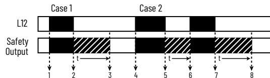
Figure 34 - Off-delay, Retriggerable Timing Diagram
