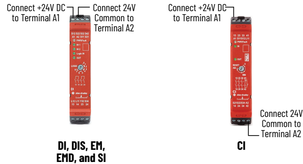
Figure 7 - Power Supply Connections
