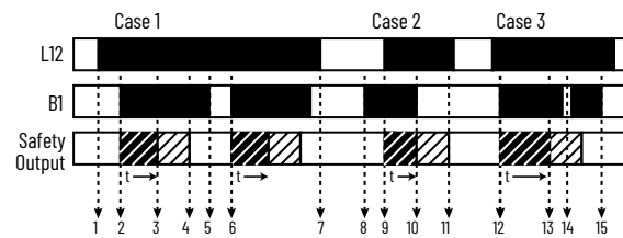
Figure 36 - Jog Timing Diagram
