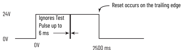
Figure 78 - Reset Input Ignores Test Pulses Up to 6 ms
