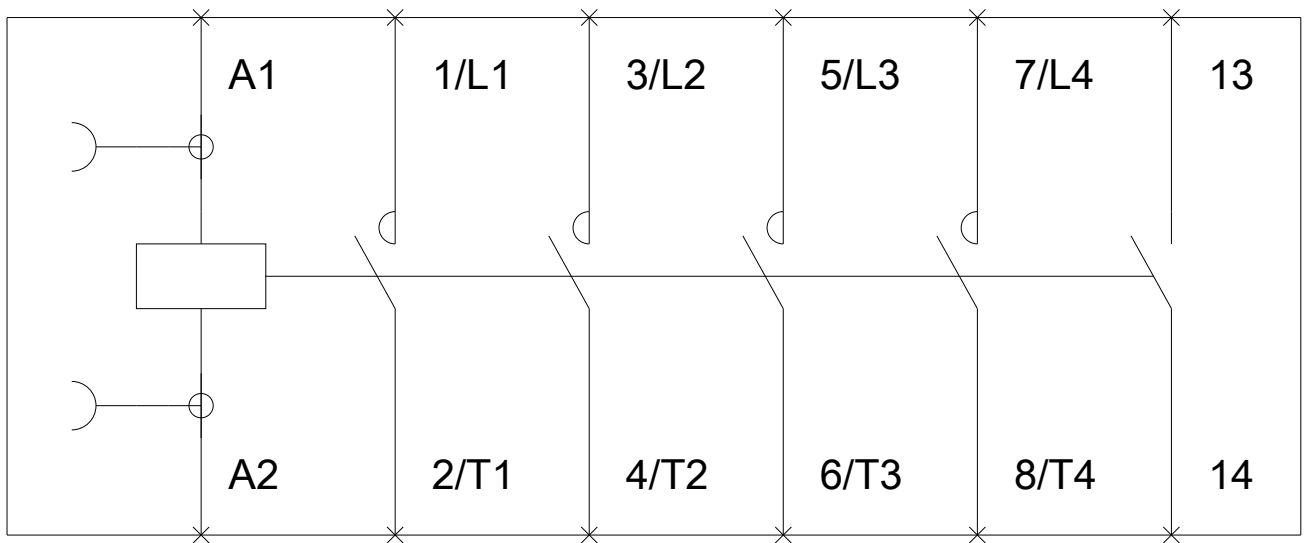
LEN00B004 Wiring Diagram
