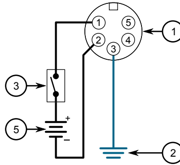
Figure 8: DC Power Supply Wiring Example (M23 Connector)
