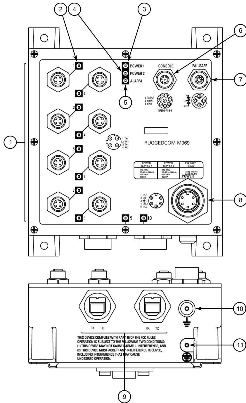
Figure 1: RUGGEDCOM M969 (M12 Connectors Shown)
