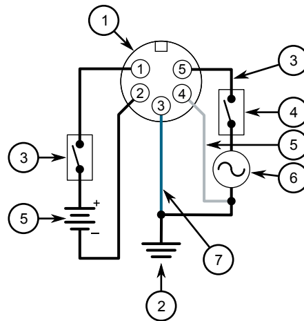
Figure 10: AC and DC Power Supply Wiring Example
