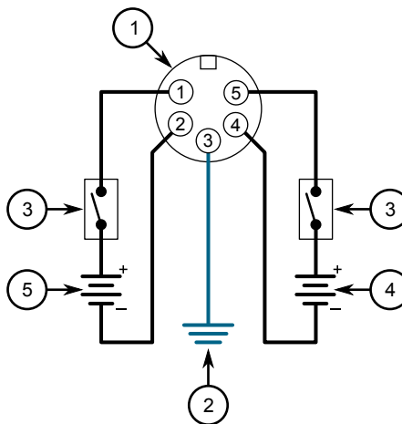
Figure 11: DC and DC Power Supply Wiring Example
