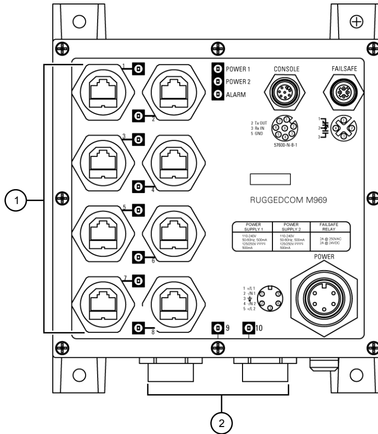
Figure 15: Port Assignment (RJ45 Connectors Shown)
