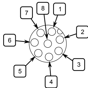
Figure 13: M12 Console Port Pin Configuration
