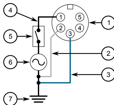
Figure 7: AC Power Supply Wiring Example (M23 Power Connector)
