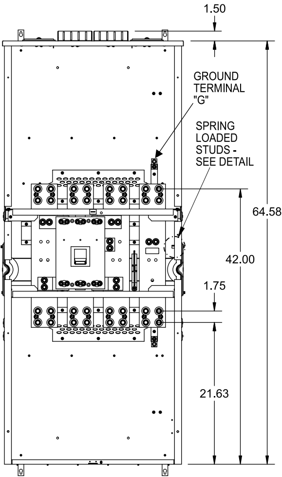
VIEW SHOWN WITHOUT COVERS
