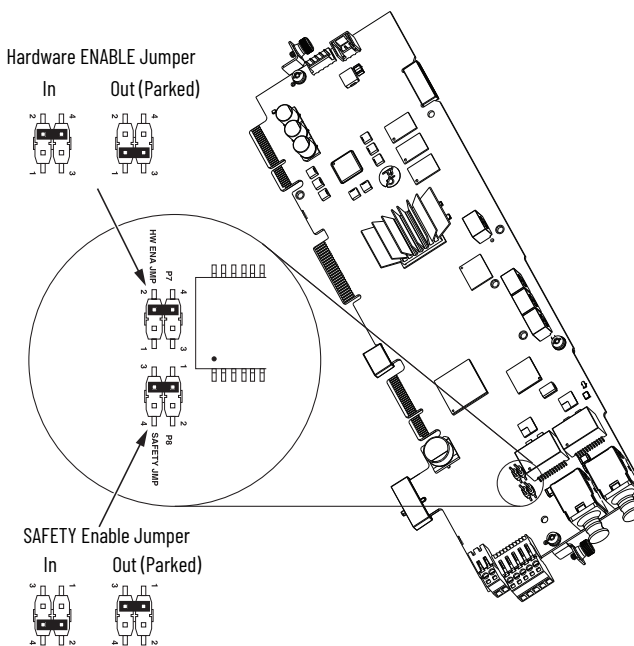
Figure 5 - PowerFlex 755TS Drives Jumper Locations
