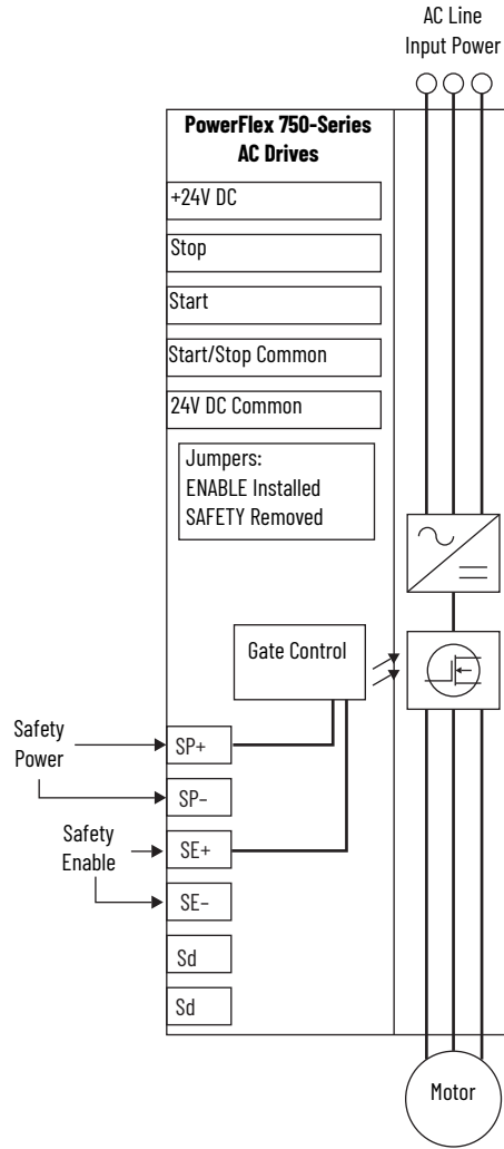
Figure 6 - Drive Safe Torque Off Circuitry
