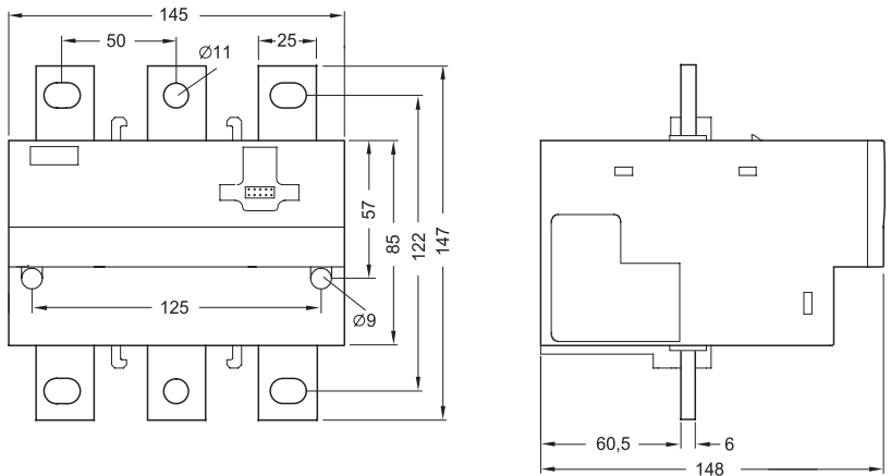
3RB29 56-2TH2 current measuring module
