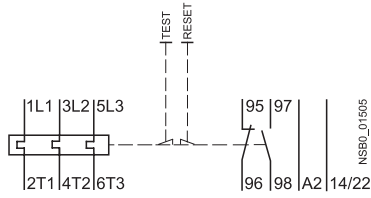
3RB30 16 overload relays
