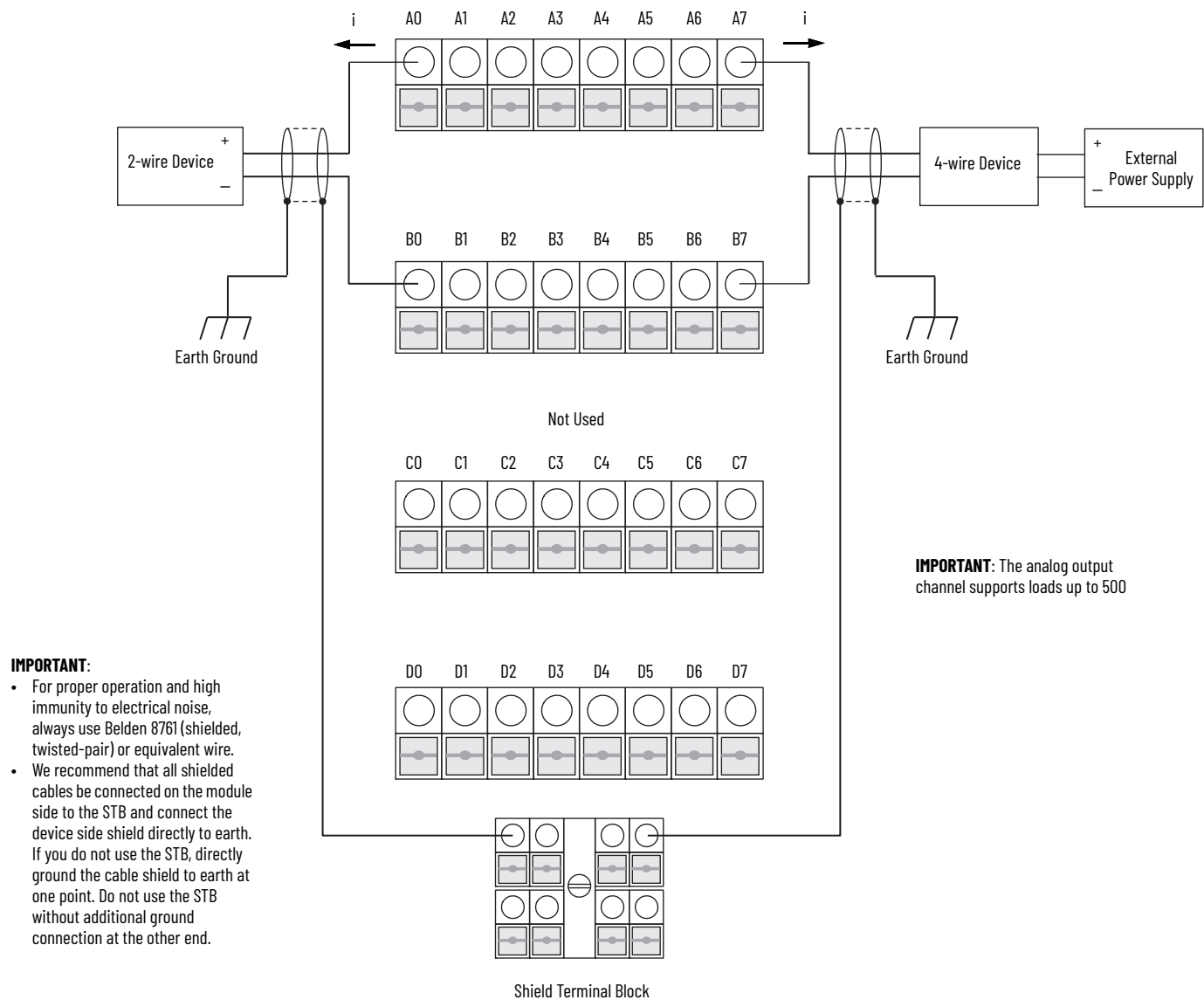
Figure 3 - Analog Outputs 2-wire and 4-wire Load
