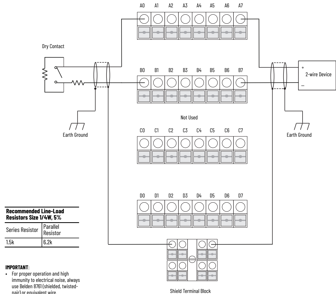
Figure 4 - Digital Inputs 2-wire Devices
