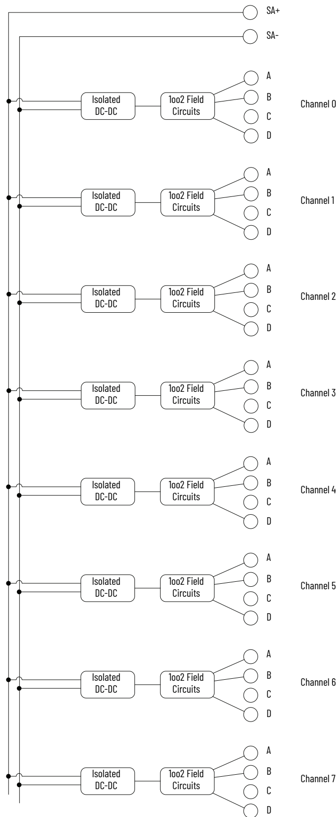
5015-U8IHFTXT Functional Block Diagram
